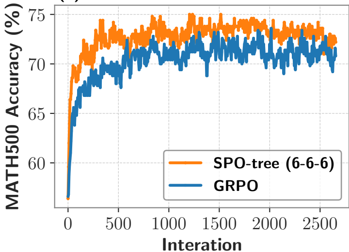
(c) Qwen2.5-Math-1.5B on MATH
